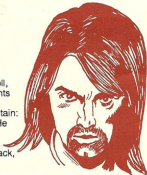
Tom Big-Mountain
